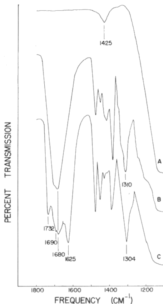
Figure 3. Infrared absorption spectra of the Al-montmorillonite diethyl succinate system
