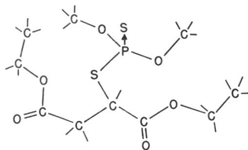
DISTANCE BETWEEN CARBOXYL OXYGENS = 4.9 Å Figure 4. Possible configuration of malathion
