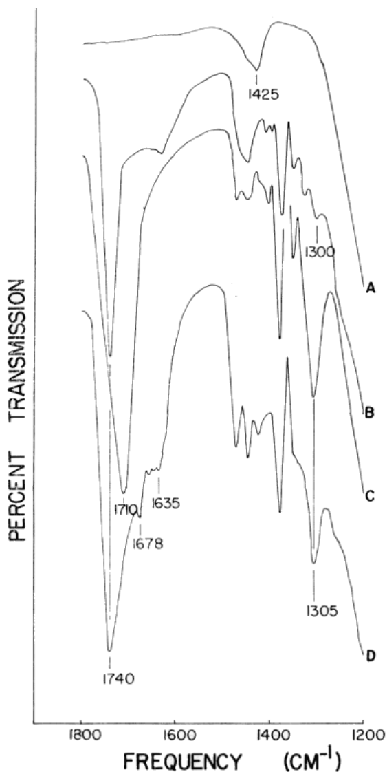
Figure 2. Infrared absorption spectra of the Al-montmorillonite-malathion system
