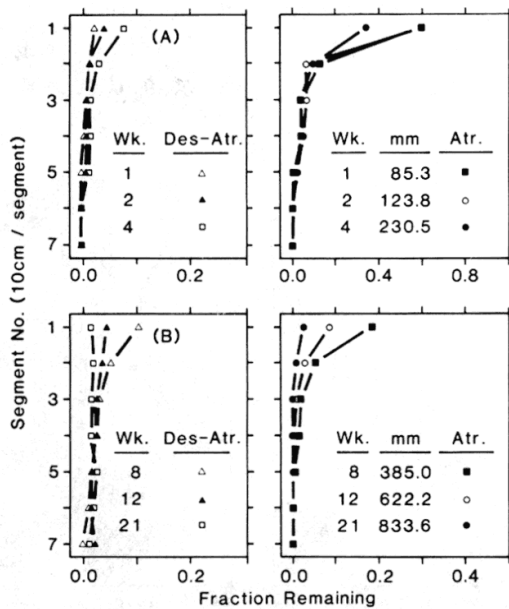
Fig. 9. Mobility profiles for atrazine and desethylatrazine in Honeywood silt loam lysimeters (isazofos-treated set) under supplementary watering. (A) Weeks 1 to 4. (B) Weeks 8 to 21. Atr. = atrazine; Des-Atr. = desethylatrazine.
