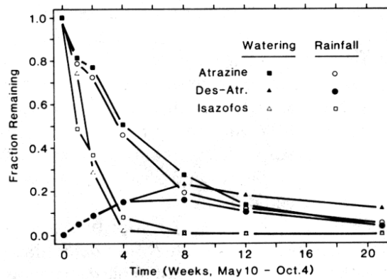
Fig. 11. Persistence of atrazine, desethylatrazine and isazofos in Honeywood silt loam lysimeters under both rainfall and supplementary watering. Des-Atr. = desethylatrazine.
