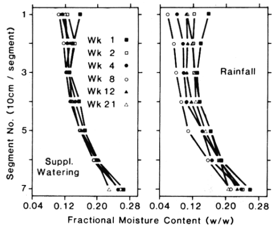
Fig. 12. Plainfield sand lysimeter moisture profiles. (A) Supplementary watering. (B) Rainfall. Saturation moisture percentage = 32.1.
