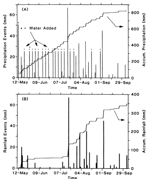
Fig. 2. London Research Centre Precipitation Record, 1988. (A) Rainfall plus supplementary watering, daily and accumulative. (B) Rainfall, daily and accumulative.
