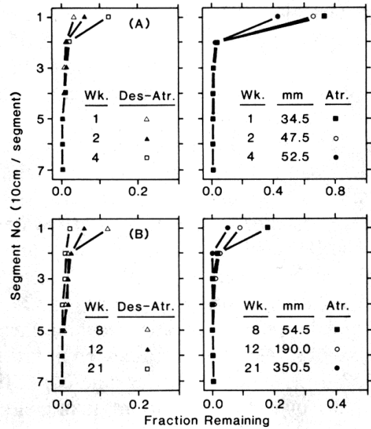
Fig. 10. Mobility profiles for atrazine and desethylatrazine in Honeywood silt loam lysimeters (isazofos-treated set) under rainfall. (A) Weeks 1 to 4. (B) Weeks 8 to 21. Atr. = atrazine; Des-Atr. = desethylatrazine.
