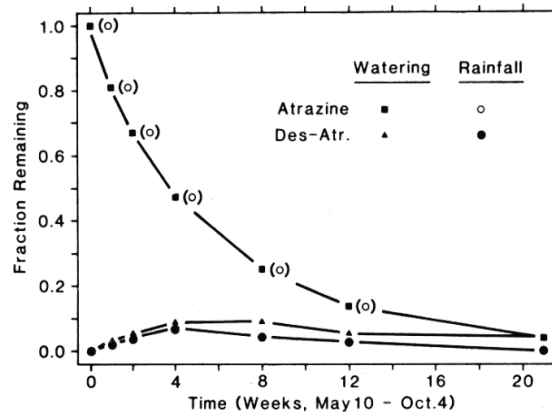
Fig. 6. Persistence of atrazine and desethylatrazine in Plainfield sand lysimeters under both rainfall and supplementary watering. Des-Atr. = desethylatrazine.
