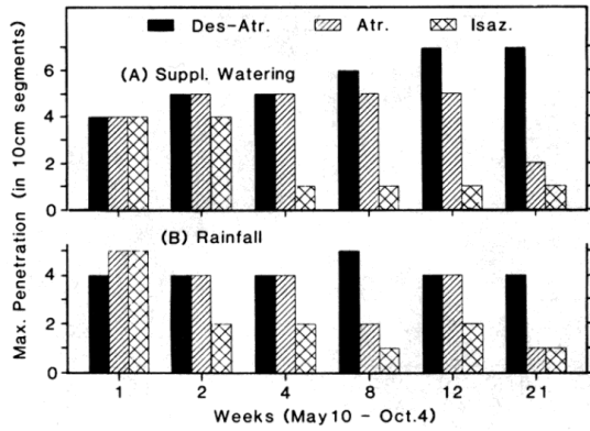
Fig. 8. Maximum penetration of atrazine, desethylatrazine and isazofos in Honeywood silt loam lysimeters. (A) Supplementary watering. (B) Rainfall. Atr. = atrazine; Des-Atr. = desethylatrazine.
