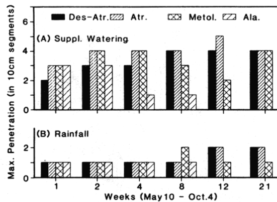
Fig. 3. Maximum penetration of alachlor, atrazine, desethylatrazine and metolachlor in Plainfield sand lysimeters. (A) Supplementary watering. (B) Rainfall. Ala. = alachlor; Atr. = atrazine; Des-Atr. = desethylatrazine; Metol. = Metolachlor.
