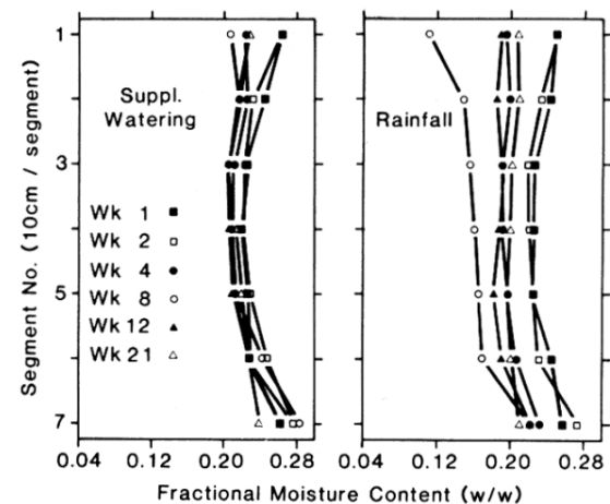
Fig. 13. Honeywood silt loam lysimeter moisture profiles. (A) Supplementary watering. (B) Rainfall. Saturation moisture percentage = 34.8.
