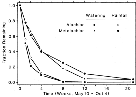
Fig. 4. Persistence of alachlor and metolachlor in Plainfield sand lysimeters under both rainfall and supplementary watering.
