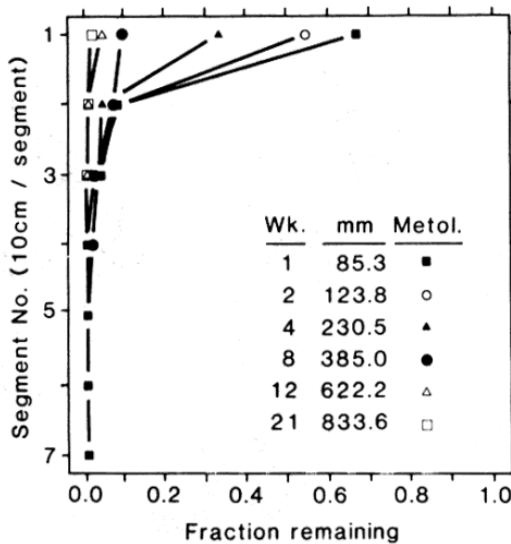
Fig. 5. Mobility profiles for metolachlor in Plainfield sand lysimeters under supplementary watering.
