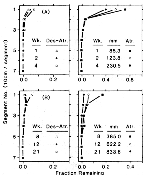
Fig. 7. Mobility profiles for atrazine and desethylatrazine in Plainfield sand lysimeters under supplementary watering. (A) Weeks 1 to 4. (B) Weeks 8 to 21. Atr. = atrazine; Des-Atr. = desethylatrazine.
