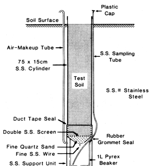
Fig. 1. Schematic representation of field-lysimeter unit.
